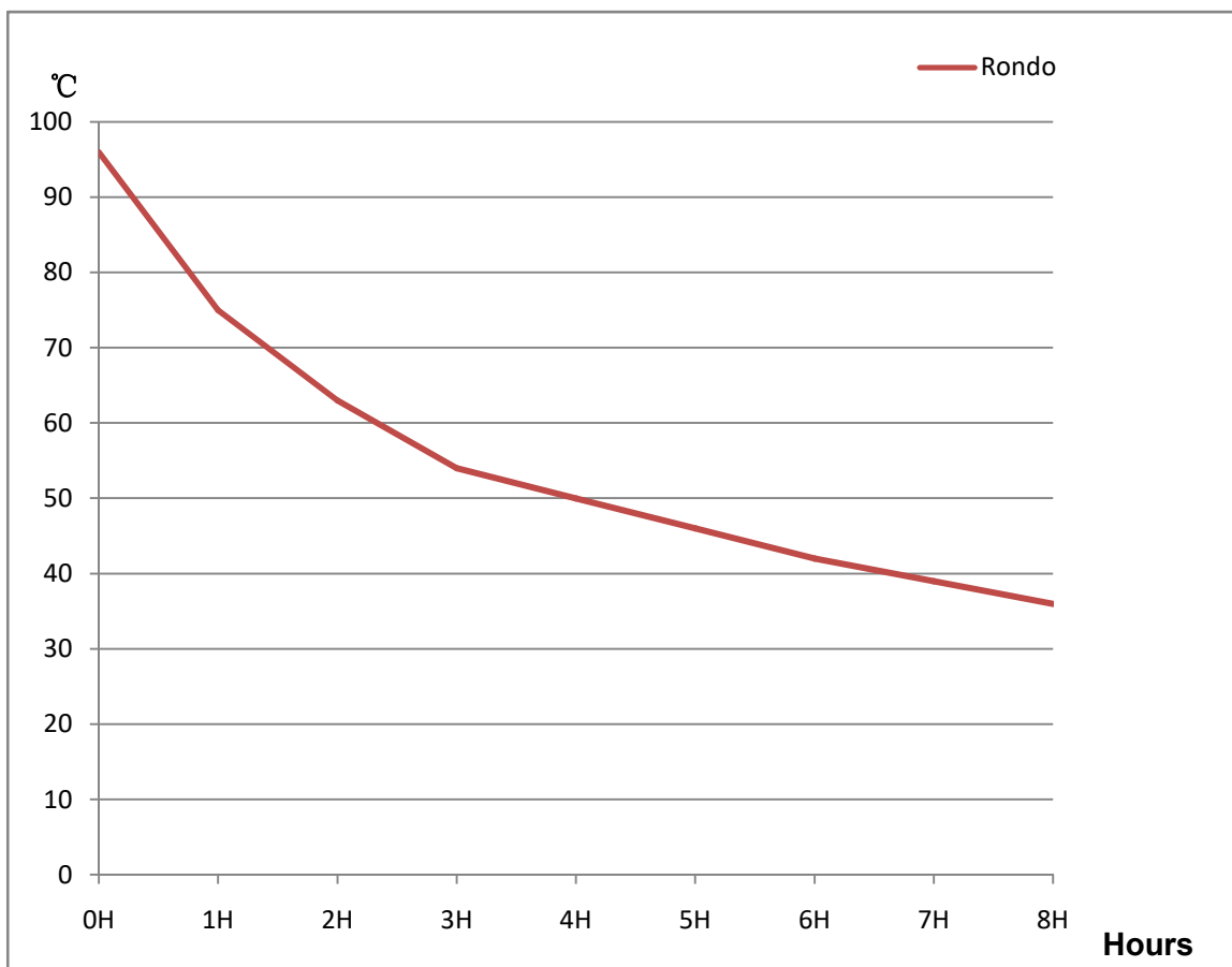
Rondo hot insulation testing
