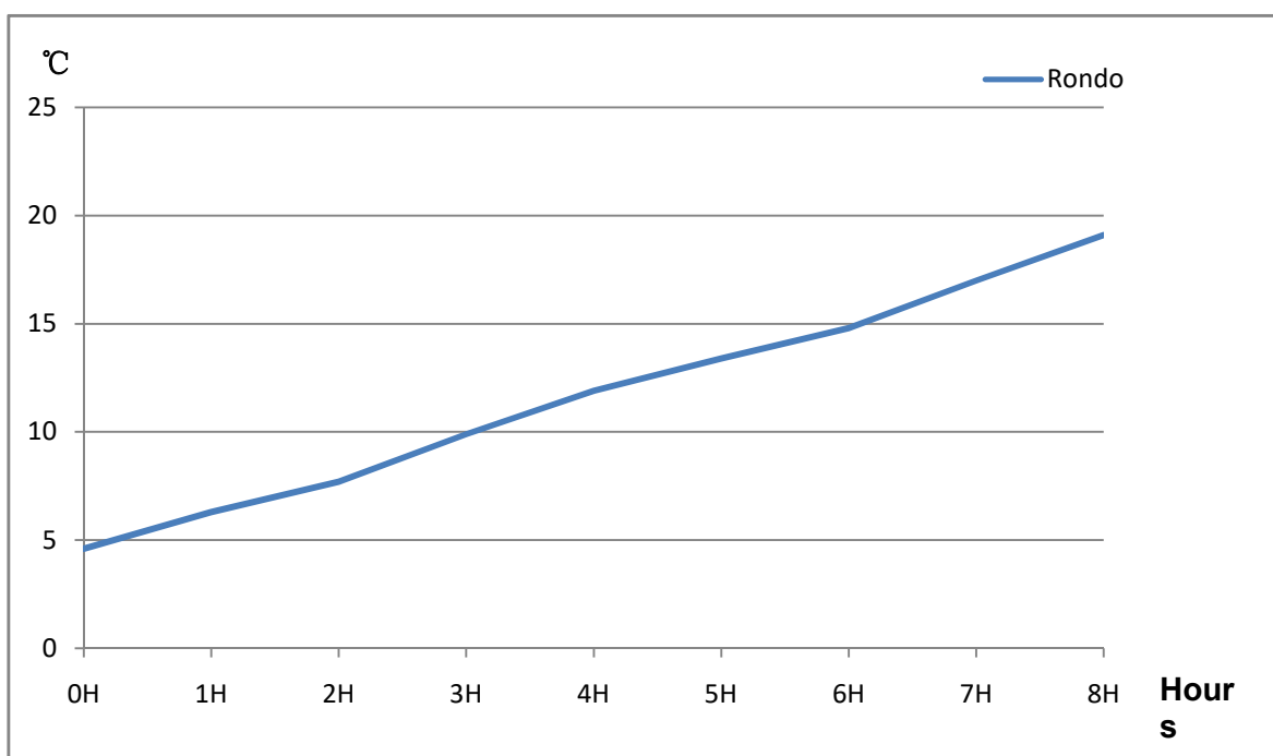
Rondo cold insulation testing
