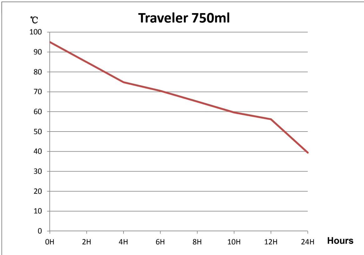
Traveler hot insulation testing
